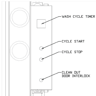
CONTROL PANEL LAYOUT DETAIL
